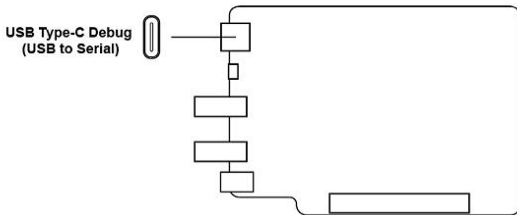
Figure 3 Debug interface
