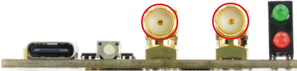
Figure 8 Antenna interface
